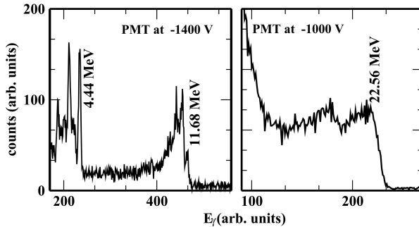
Fig. 2. Parts of gamma ray spectra measured by LaBr 3 :Ce in the ^{11}\text{B}(p,\gamma)^{12}\text{C} reaction; Gamma lines of 11.68 MeV and 22.56 MeV are indicated.
