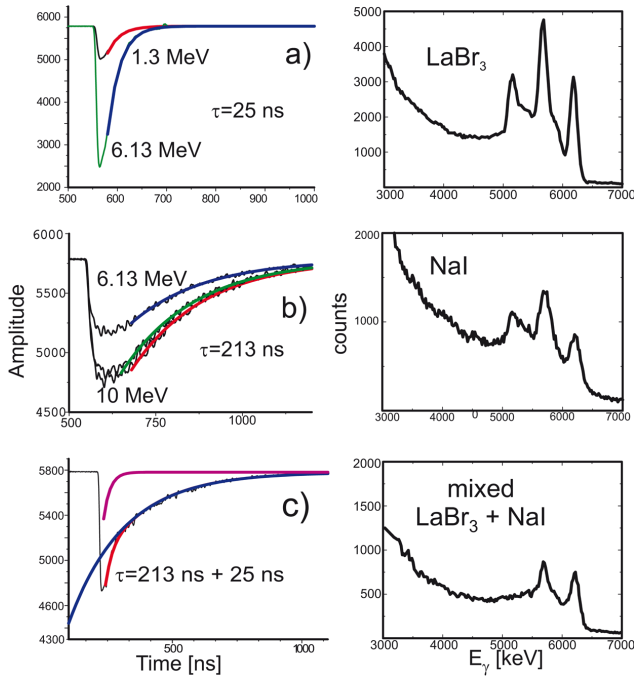
Fig. 5. Left: the analytical function fit to signal shapes associated with different regions of the Qfast–Qslow matrix, as indicated in Fig. 4 (left). Calculated decay times \tau are shown. Right: the 6.13 MeV gamma line and the escape peaks reconstructed by charge integration of the filtered detector pulses.
