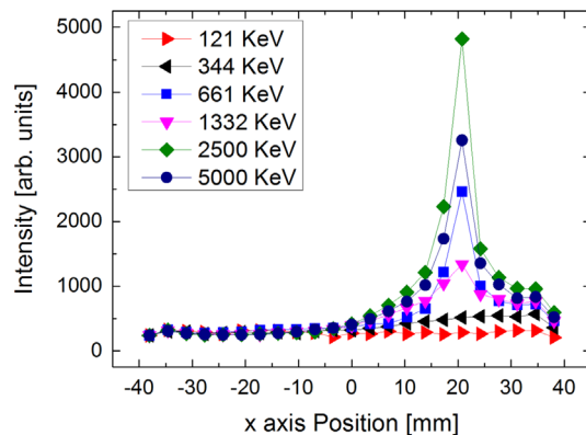
Fig. 6. Intensity distribution of the scintillation light as measured on the photocathode for gamma rays of energy from 121 keV up to 5 MeV. In the left panel the source is in position (x, y)=(0 \text{ cm}, 0 \text{ cm}) , in the right panel the source is in position (x, y)=(2 \text{ cm}, 0 \text{ cm}) and in both plots the curves have been normalized to have the same intensity at x=-40 \text{ mm} .
