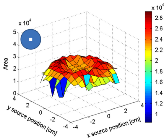
Fig. 11. The area of the full energy peak is shown as a function of the source position. The window was placed at the center of the photocathode, as indicated in the inset. For a clearer view colors were introduced, the color legend is on the right side and refers to the area (z-axis).
