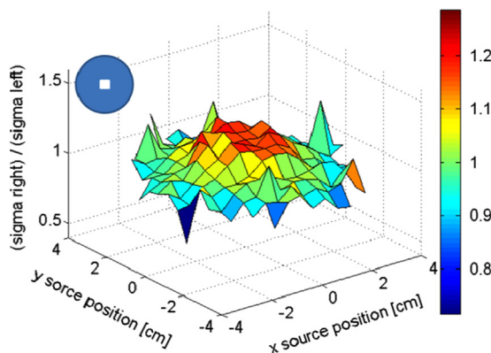
Fig. 12. The ratio of sigma left and sigma right is shown as a function of the source position. The window was placed at the center of the photocathode, as indicated in the inset. For a clearer view colors were introduced, the color legend is on the right side and refers to the sigma left and sigma right ratio (z-axis).
